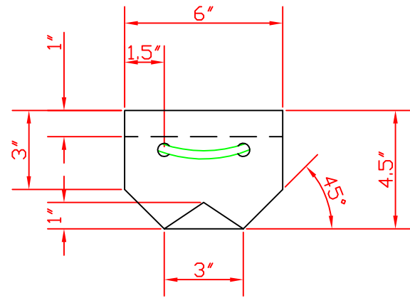
FLEX ANCHOR
