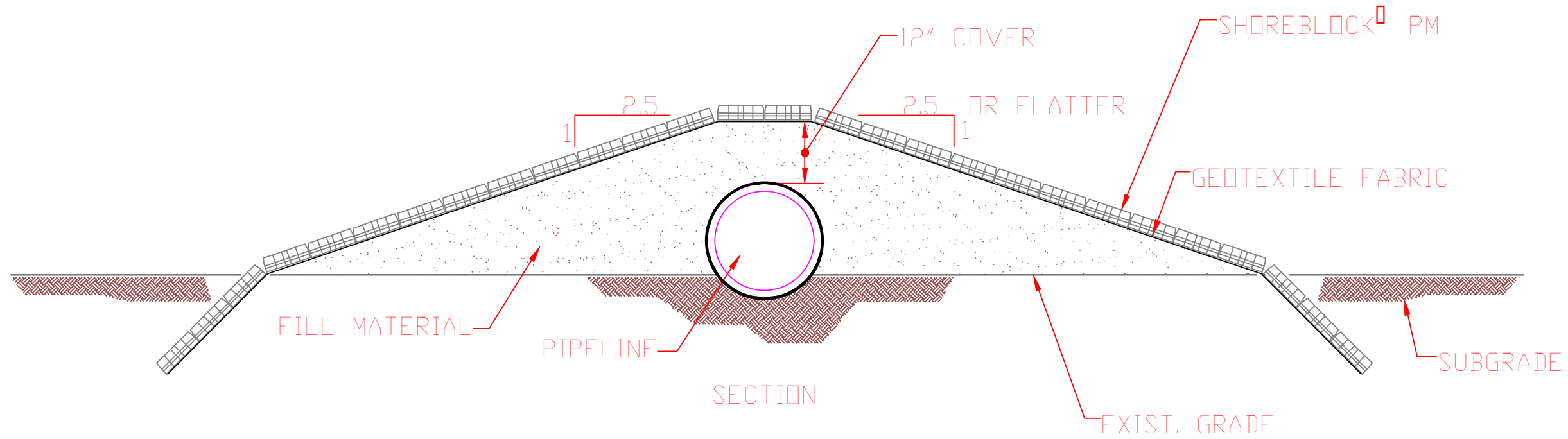
PIPELINE COVER SECTION
