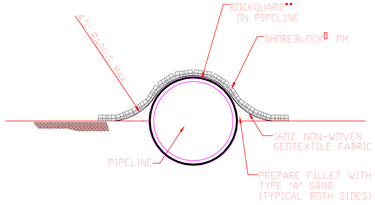
PIPELINE COVER SECTION
